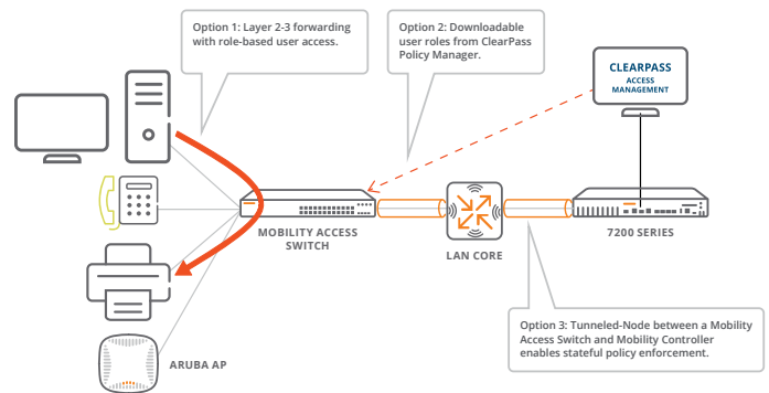
Figure 1. Flexible secure wired access deployments
