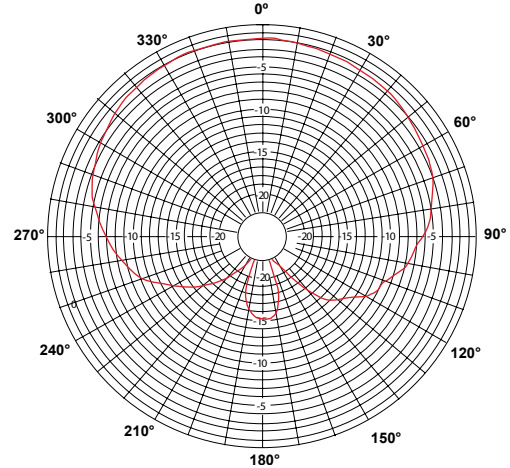
AZIMUTH PLANE - 2450MHZ
