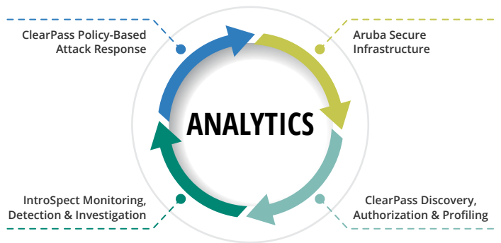
Figure 3: Analytics-driven security
