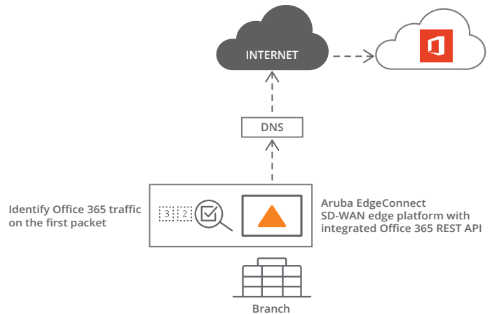
Figure 1: Local Egress of Office 365 using Aruba EdgeConnect SD-WAN
